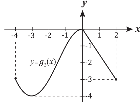
Figura 10: g_3
